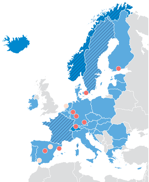
Figure 4.5 SAF supplied in Europe, March 2022
