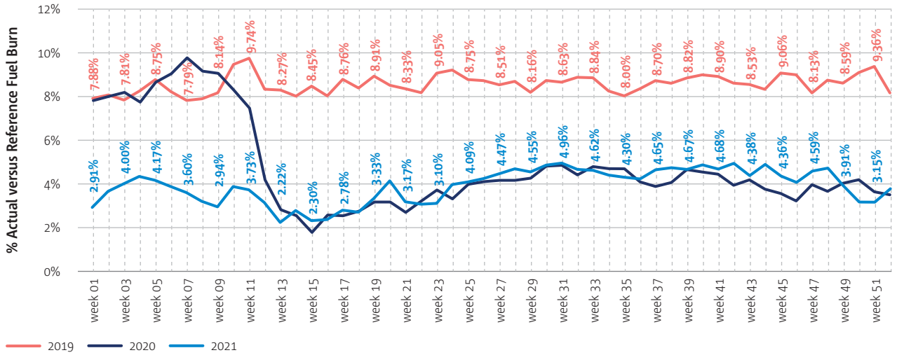
Figure 5.5 Intra-NM Area 43 proportion of excess fuel burn (kg) – XFB10
