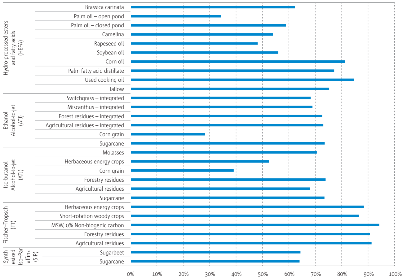
Figure 4.3 LCA emissions reductions for CORSIA eligible SAF pathways and feedstock compared to a fossil fuel reference value (89 g CO 2 e/MJ) [11] 38
