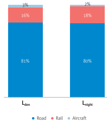
Share of people exposed to harmful noise levels by transport mode (2017, EU27+EFTA)
